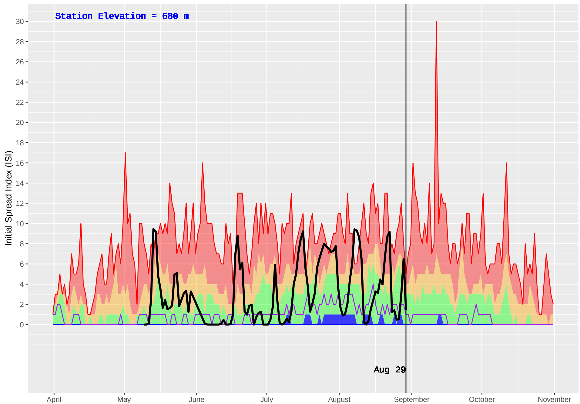
SUMMIT (11) : Historical (1985–2016) and Current (2018) Daily Initial Spread Index (ISI)
